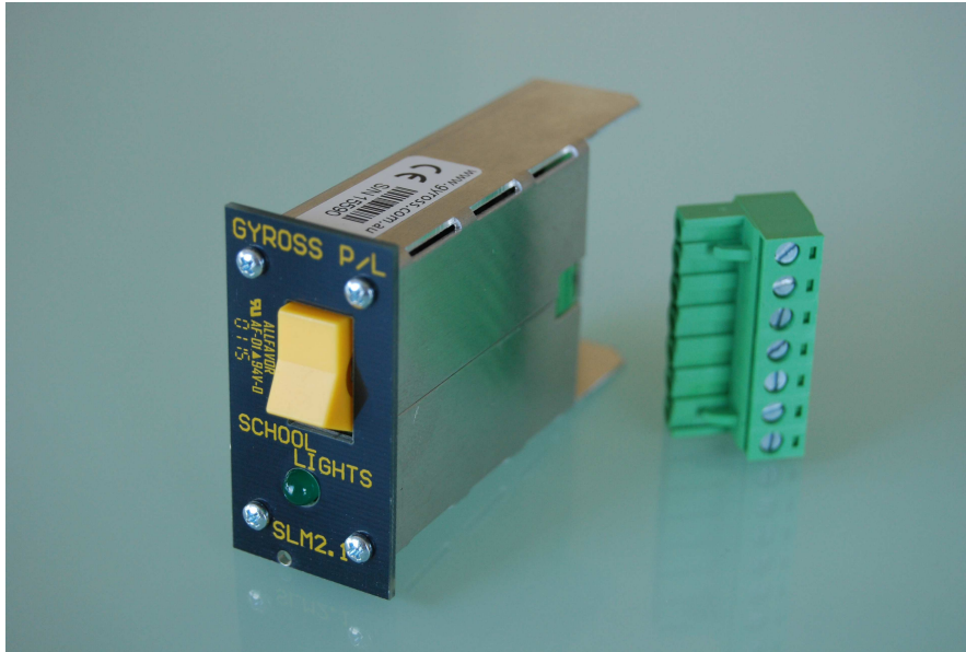
School Light Module for amber lights
